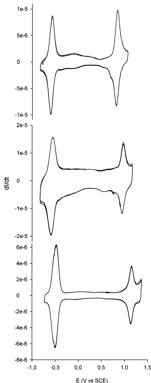
FIGURE 2. Deconvoluted CV of compounds 6 , 5 , and 4 (from top to bottom) in \text{CH}_2\text{Cl}_2 , TBAPF 6 0.1 M 100mV/S vs SCE.
