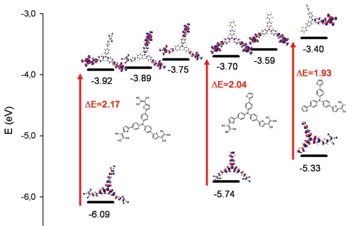
FIGURE 3. Calculated HOMO and LUMO levels for compounds 4–6.
